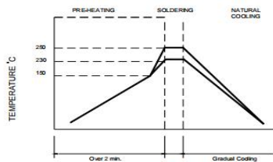
Figure 2. Wave Soldering
