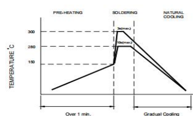
Figure 3. Hand Soldering
